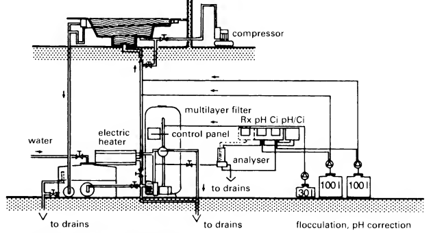
④ Whirlpool servicing diagram
